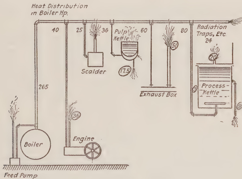
FIG. 1 TYPICAL STEAM DISTRIBUTION
